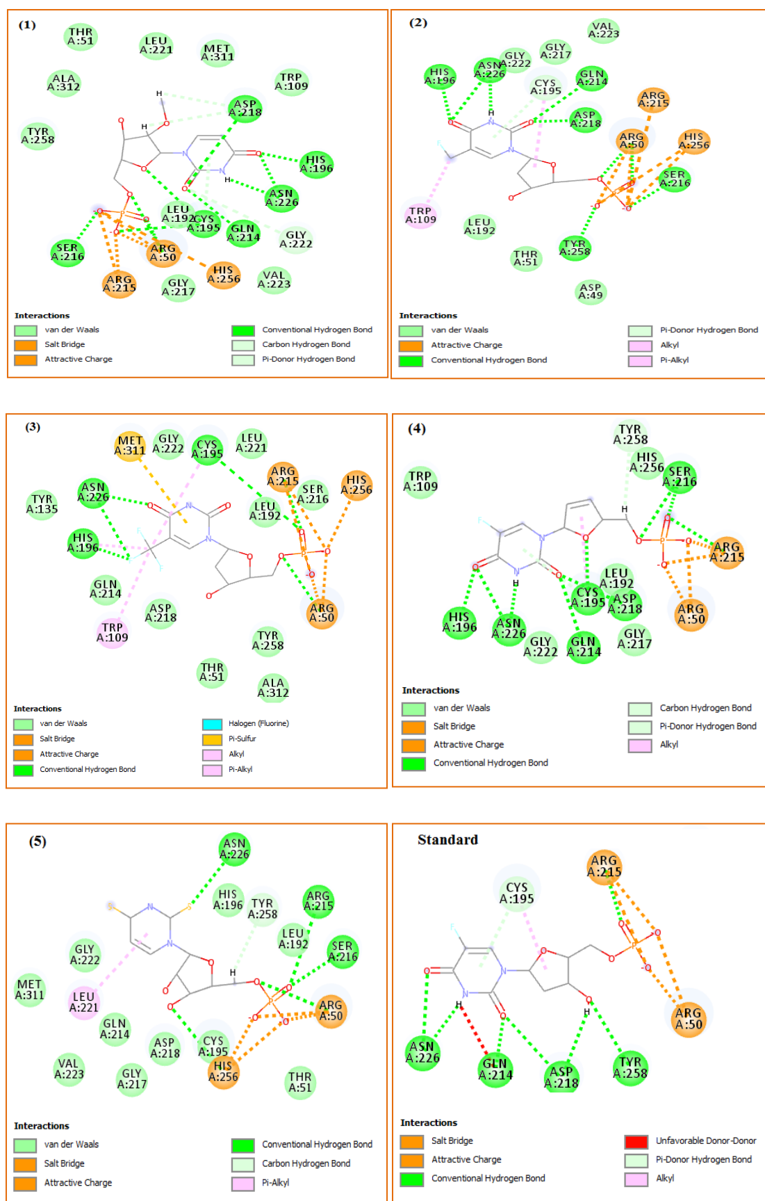
Figure 1: Interaction diagrams showing compounds 1-5 and standard drug in complex with hTS (PDB code: 1hvy).
