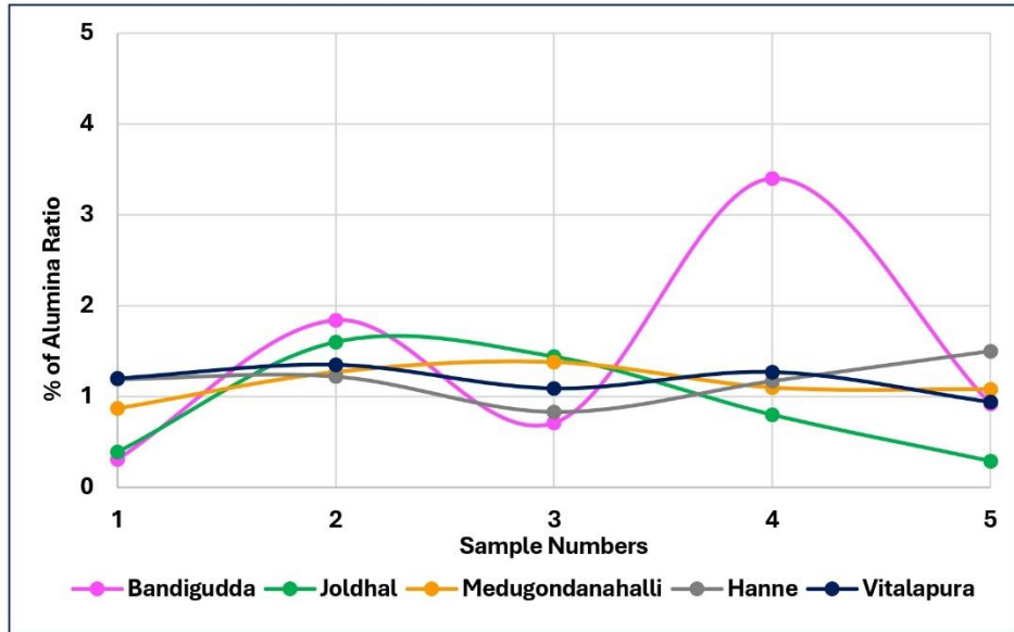
Figure 11 Illustrate average Alumina modulus of all five region collected limestone samples from the study area
