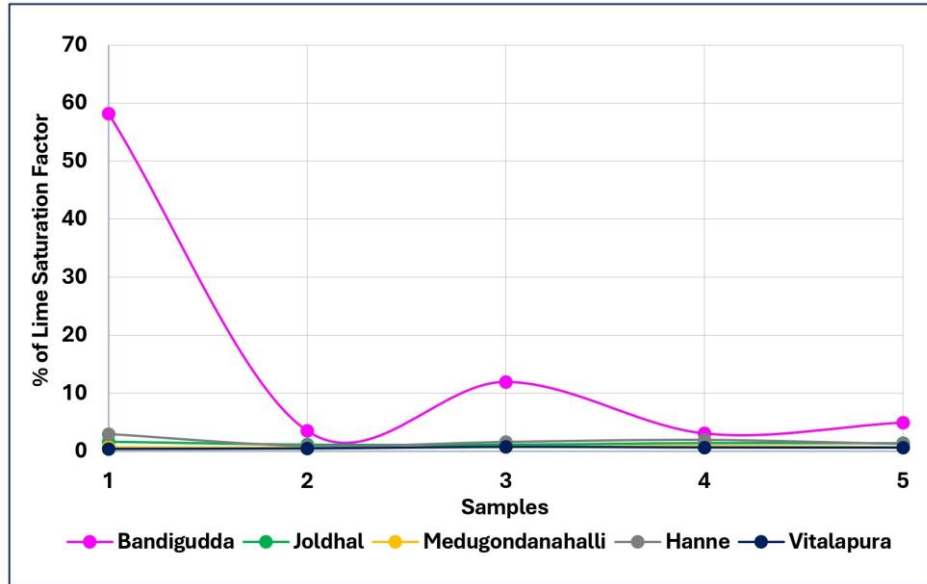
Figure 9 Illustrate average lime saturation factor of all five region collected limestone samples from the study area
