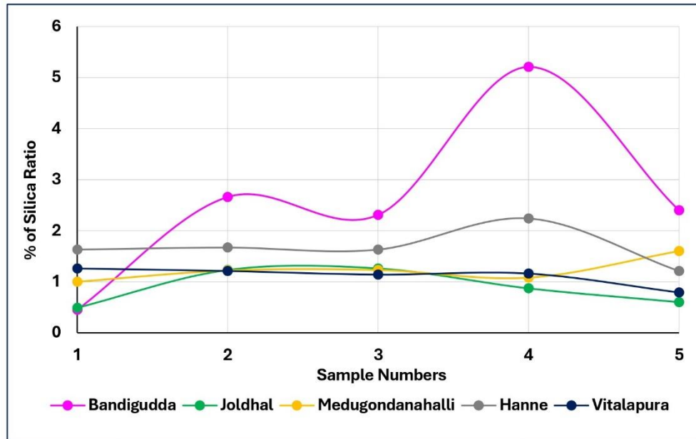
Figure 13 Illustrate average silica modulus of five region collected limestone samples from the study area
