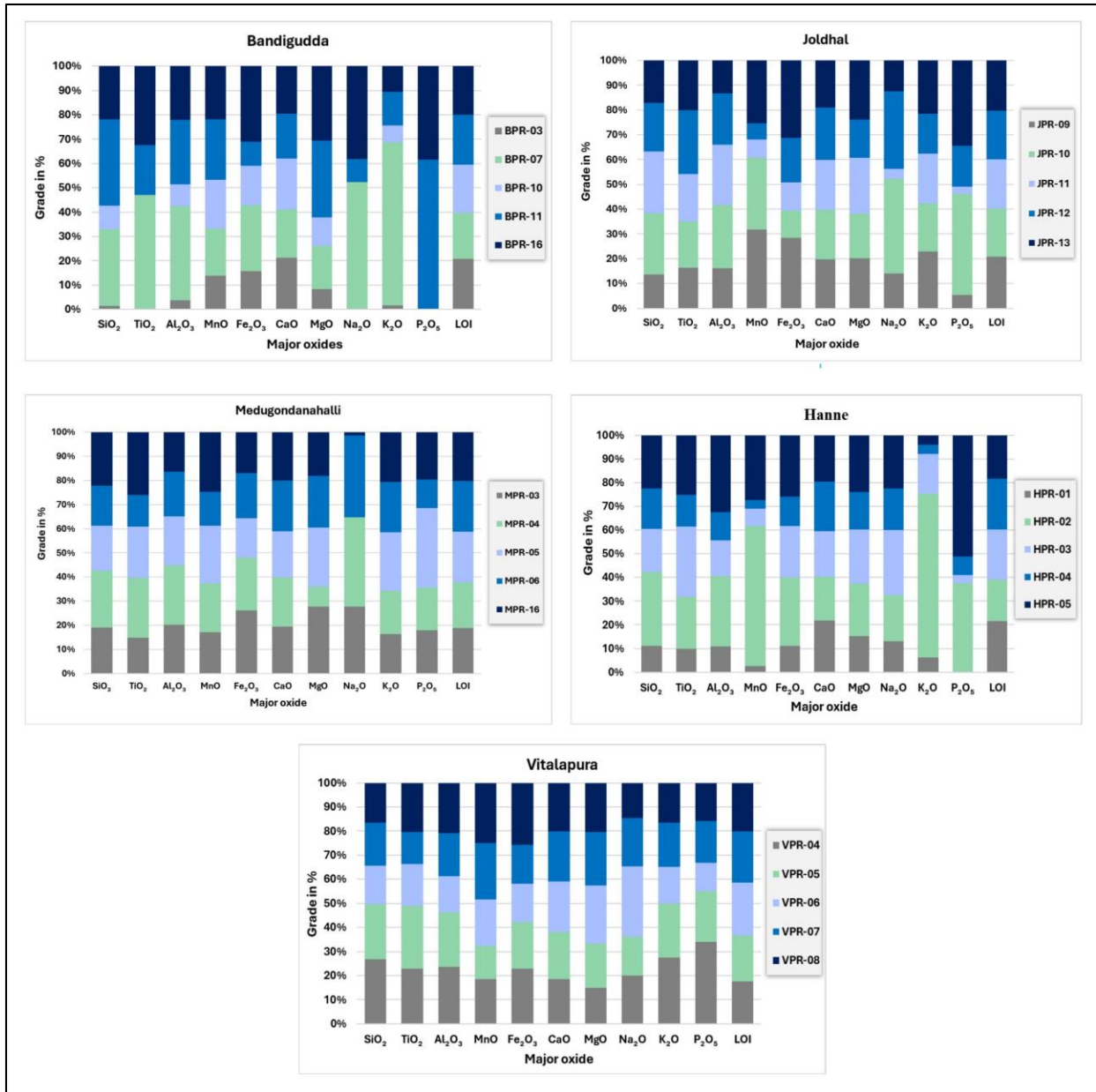
Figure 7 Represent the grade concentration % of major oxide various region of the study area
