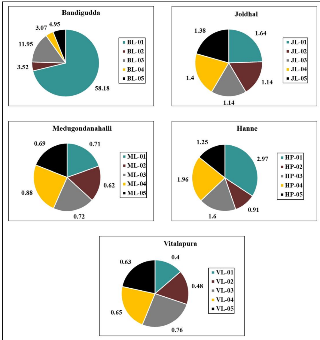
Figure 8 Illustrate lime saturation factor of all 5 regions collected limestone samples from the study area
