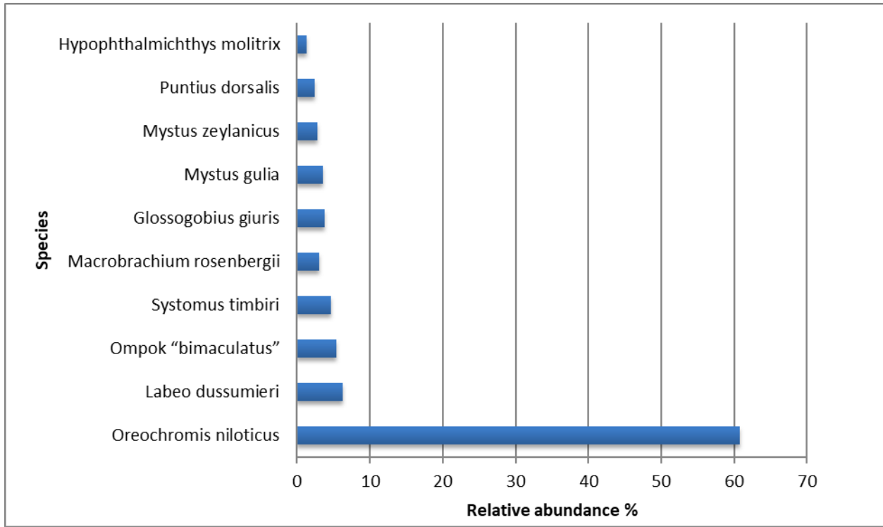
Figure 2 Relative Abundance of 10 most common fish species of vawnikulam reservoirs - (sorted by abundance).
